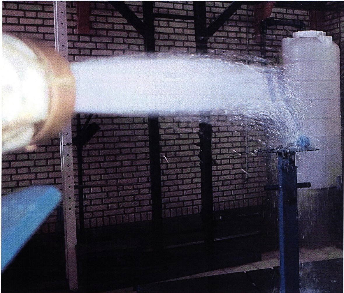
Figure 3: EUT under IPX6
