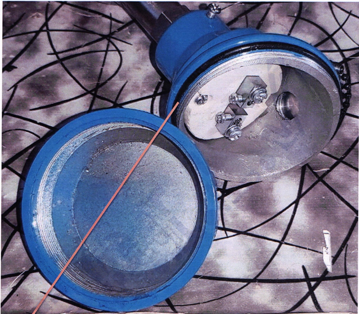
Figure 4: EUT after IPX7
