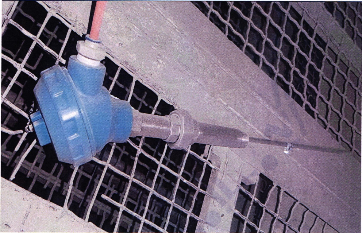
Figure 2: EUT after IP6X
